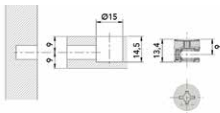
Excenter kastverbinding type 21306010ZN
